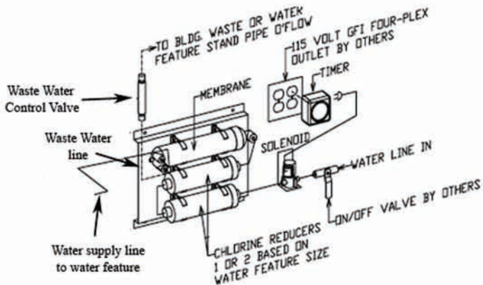
Reverse Osmosis System Setup
